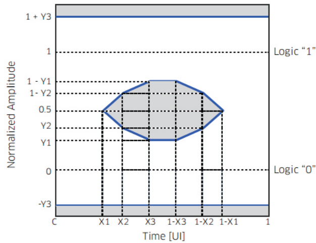
Mask of optical output eye diagram
